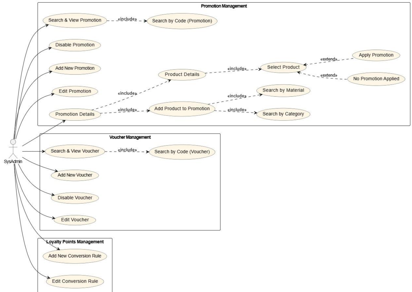
Hình 17. Draw the usecase of Promotion/Voucher/Loyalty Points Management
